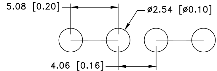
MOUNTING DETAIL
