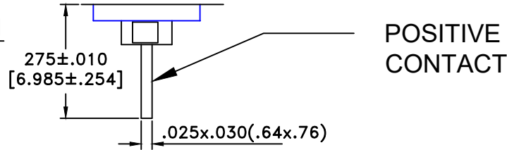
Square Contact Detail
